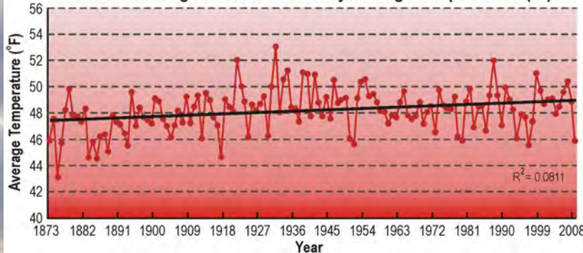
Figure 2-5. Annual average of state-wide daily average temperatures (°F) from 1873-2008. Note the increase in the first half of the 20th century and little change since then. Seasonal and day-night changes are proportionately larger and have greater impacts – with winter and nighttime temperatures increasing more than summer and daytime temperatures. (Data from Iowa Climatology Bureau 2010.)
