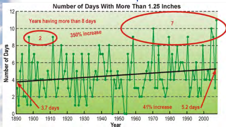
Figure 2-4. Annual number of days when daily total precipitation exceeded 1.25 inches (3 cm) in Des Moines. Note the increase in number of years having more than 8 days with daily total precipitation exceeding 1.25 inches. (Data from Iowa Climatology Bureau 2010.)
